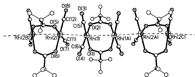
Fig. 1 A perspective view of [\text{Rh}_2(\mu\text{-O}_2\text{CCF}_3)_2(\text{CO})_4]_n ( 2 ). Selected distances (Å) and angles (°): Rh(1)–Rh(1A) 2.984(1), Rh(1)–Rh(2) 3.092(1), Rh(2)–Rh(2B) 2.994(1), Rh–O 2.087(5), Rh–C 1.839(9); Rh–Rh–Rh 162.23(1), O–Rh–O 85.2(2), C–Rh–C 89.0(4), Rh–Rh–O 79.6(2), Rh–Rh–C 101.4(3).
