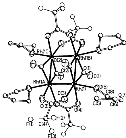
Fig. 2 A perspective view of [\text{Rh}(\mu\text{-O}_2\text{CCF}_3)(\mu\text{-CO})(\text{THF})_4]_4 ( 3 ). Selected bond distances (Å) and angles ( ^\circ ): Rh(1)–Rh(1A) 2.551(1), Rh(1)–Rh(1B) 2.624(1), Rh–C 1.959(8), Rh–O 2.153(6), Rh–O THF 2.220(5); Rh–Rh–Rh 90.0, O–Rh–O 82.4(3), C–Rh–C 95.1(3), Rh(1A)–Rh(1)–O 85.5(2), Rh(1A)–Rh(1)–C 94.8(3), Rh(1A)–Rh(1)–O THF 169.8(2), Rh–C–Rh 84.1(4).
